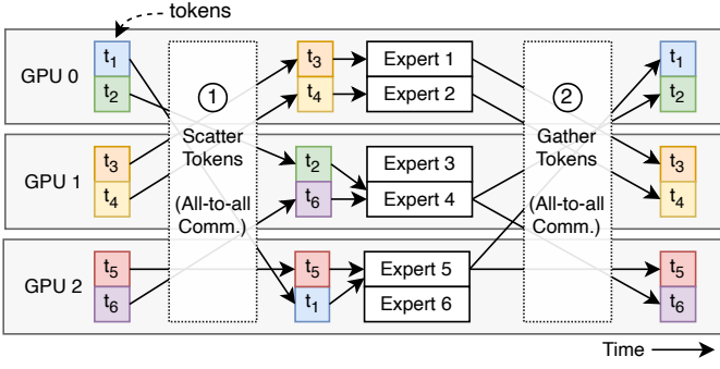
Fig. 3: Token scattering (step 1) and gathering (step 2) when using expert parallelism. Experts are split across GPUs. One batch requires two all-to-all synchronization barriers.
