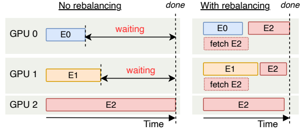
(b) Timeline with operations per GPU, with and without rebalancing. Experts are fetched asynchronously (see Section IV-C).
